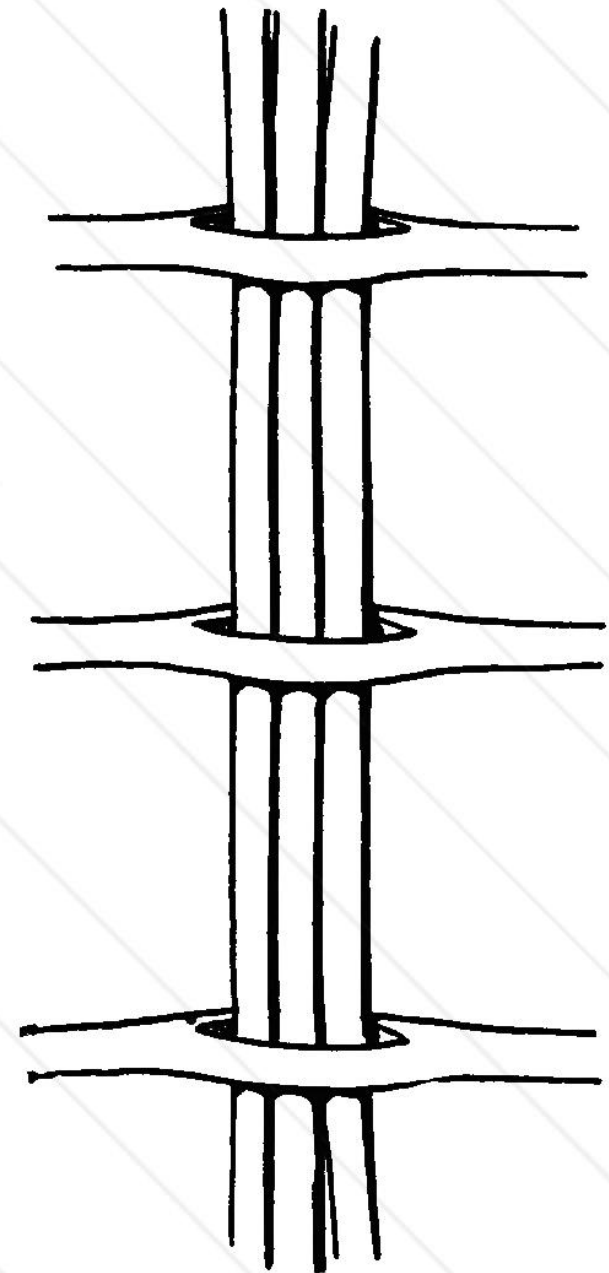
The Short Spokes are Split and the Long Ones Slipped Through
